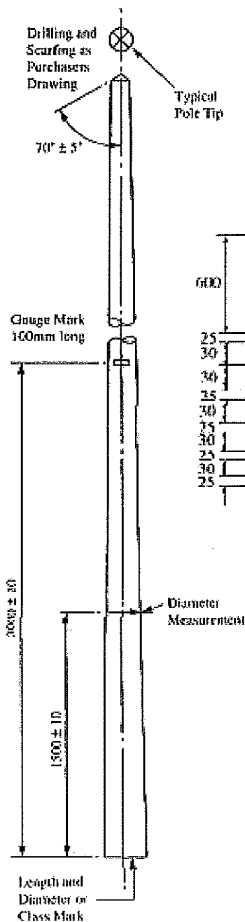
Typical layout
